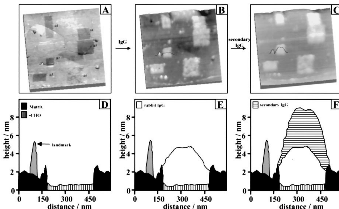
FIGURE 4 Recognition (binding) of specific mouse-anti-rabbit IgG onto nanopatterns of rabbit IgG. (A) Nanopatterns of 3-mercaptopropional with sizes 500 \times 200 \text{ nm}^2 , 200 \times 200 \text{ nm}^2 , 300 \times 180 \text{ nm}^2 , 300 \times 300 \text{ nm}^2 , and 350 \times 350 \text{ nm}^2 , a1–a5, were produced within a 1500 \times 1500 \text{ nm}^2 area of 1-dodecanethiol SAM. An incomplete pattern formed by using a smaller fabrication force is shown in the bottom right corner, a6. (B) The same area after the patterns were immersed in a 0.01 mg/ml solution of rabbit IgG for 3 min followed by washing with 1% Tween 20 solution. (C) After introducing mouse anti-rabbit IgG, the patterns display an increase in height, indicating the specific binding of antibody to the immobilized protein. (D–F) Corresponding cursor profiles drawn in the same position for images A–C. The feature (colored gray) beside pattern a2 is used as a reference to illustrate the height increases after rabbit IgG adsorption and after binding of mouse anti-rabbit IgG.
