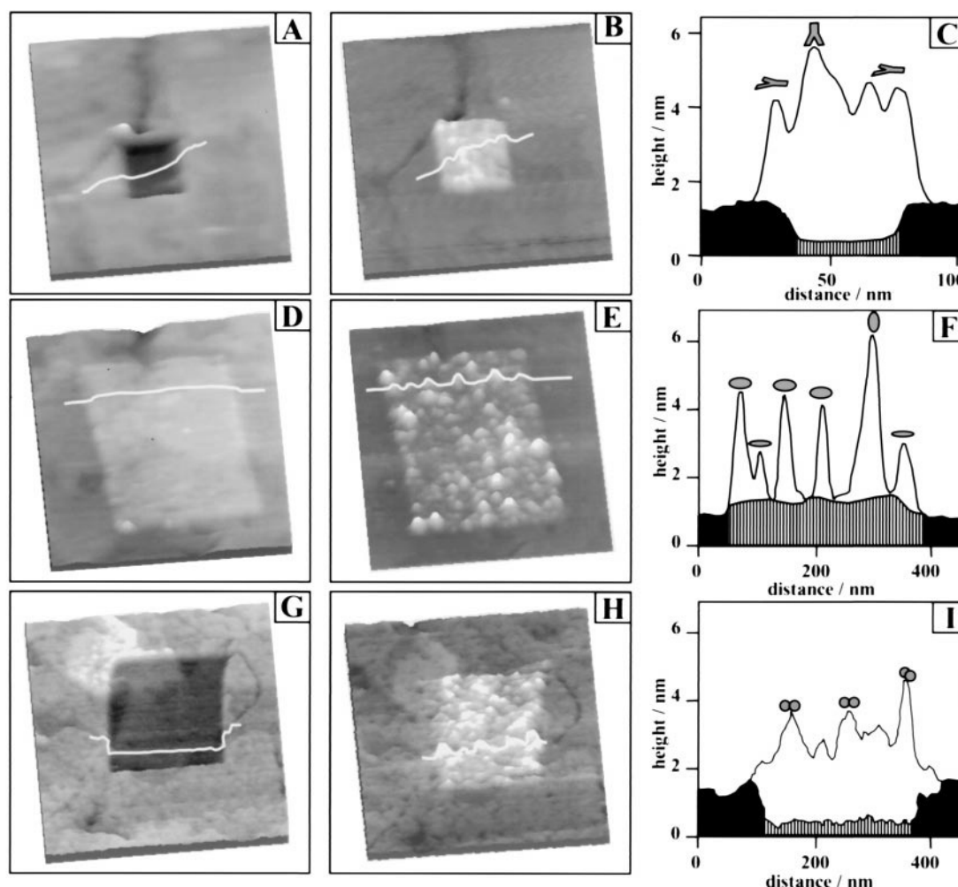
FIGURE 3 Production of nanopatterns of IgG, LYZ, and BSA via covalent binding. (A) A 150 \times 150 \text{ nm}^2 topographic image with a 40 \times 40 \text{ nm}^2 pattern of 3-mercaptopropional in a decanethiol SAM matrix; (B) The same pattern after IgG adsorption; (C) The combined cursor profile of images A and B; (D) A 600 \times 600 \text{ nm}^2 topographic image of a hexanethiol SAM matrix, with a 350 \times 300 \text{ nm}^2 nanografted pattern of 11-mercaptopropional; (E) The same area imaged after LYZ adsorption; (F) The combined cursor profile of images D and E; (G) A 600 \times 600 \text{ nm}^2 topographic image of a hexanethiol SAM, with a 200 \times 250 \text{ nm}^2 nanopattern of 3-mercaptopropional; (H) The same area imaged after immobilization of BSA; (I) The combined cursor profile of G and H.
